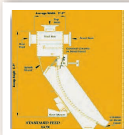
The Deister Sieve Bend is used in various applications in Preparation Plants where coal is wetted and processed.
