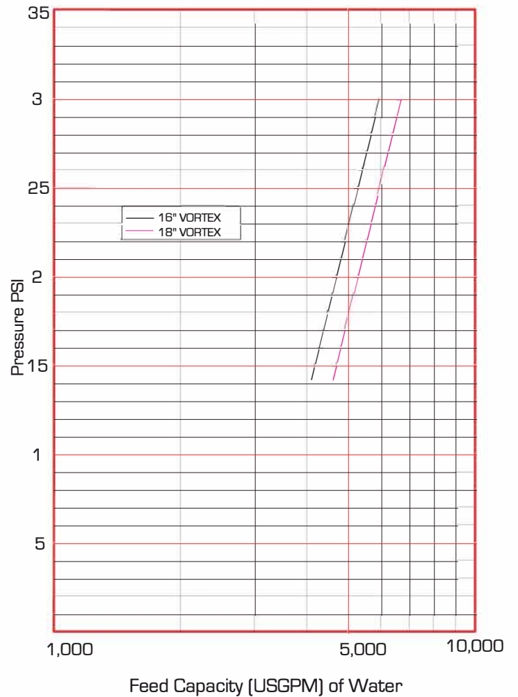
Deister- Model C-42-B-20FB Heavy Medium Cyclone 132.7 Sq. in. (85, 613 Sq. mm) Inlet
