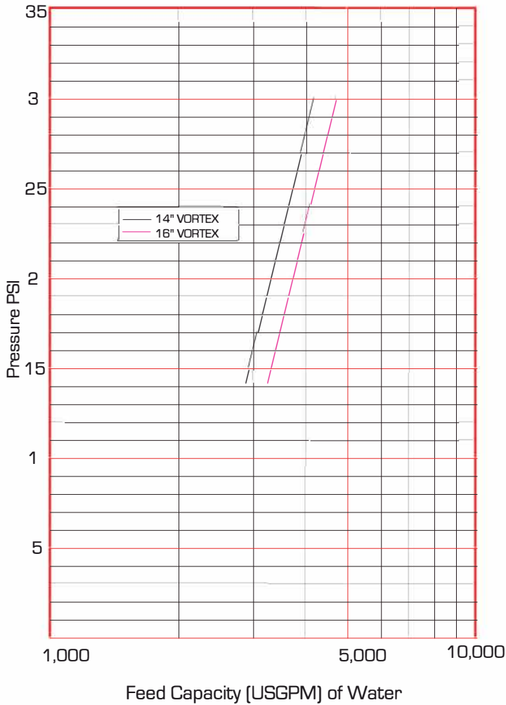
Deister- Model C-42-B-20FA Heavy Medium Cyclone 86.5 Sq. in. (56, 585 Sq. mm) Inlet
