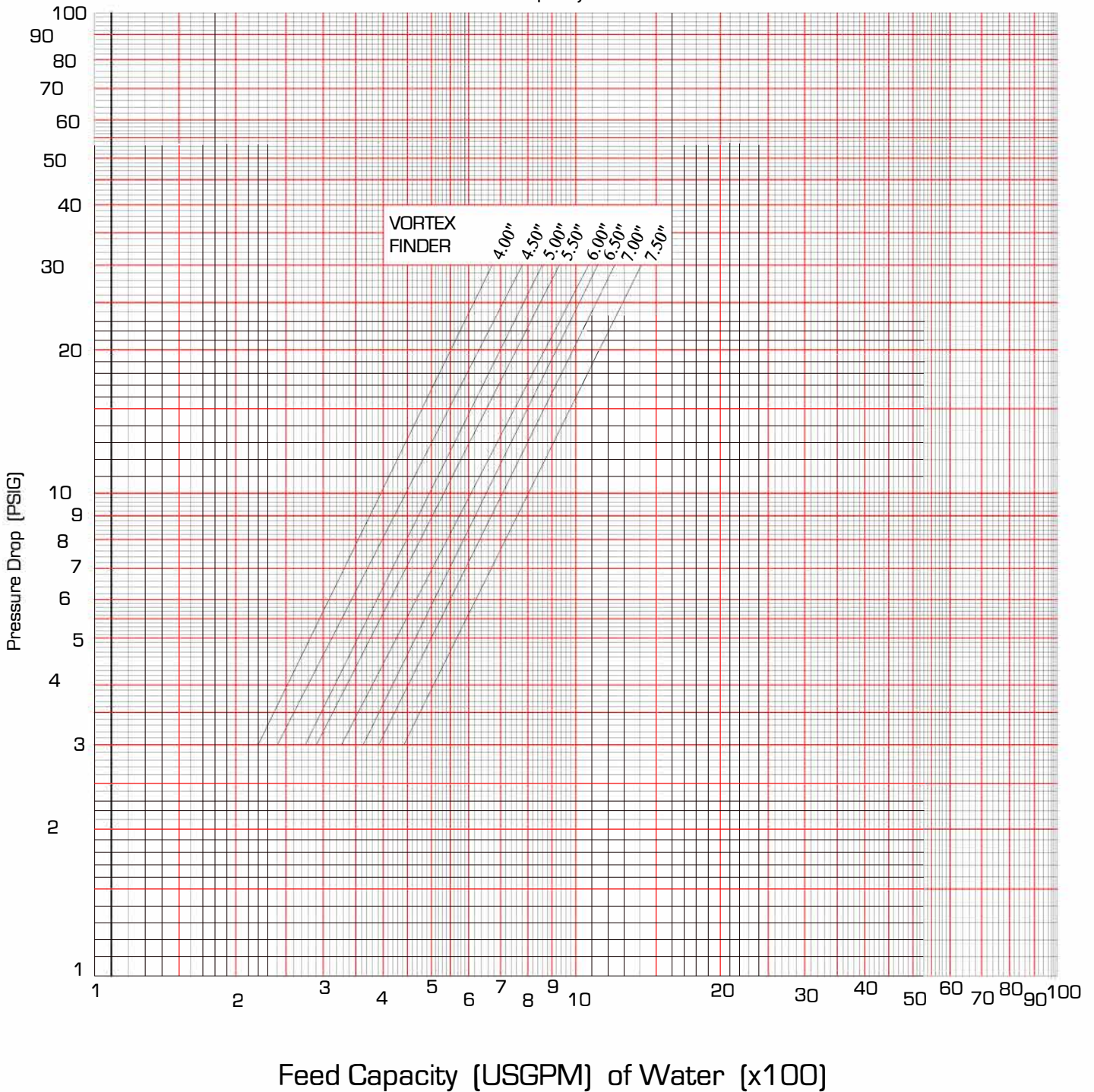
Capacity Curve
