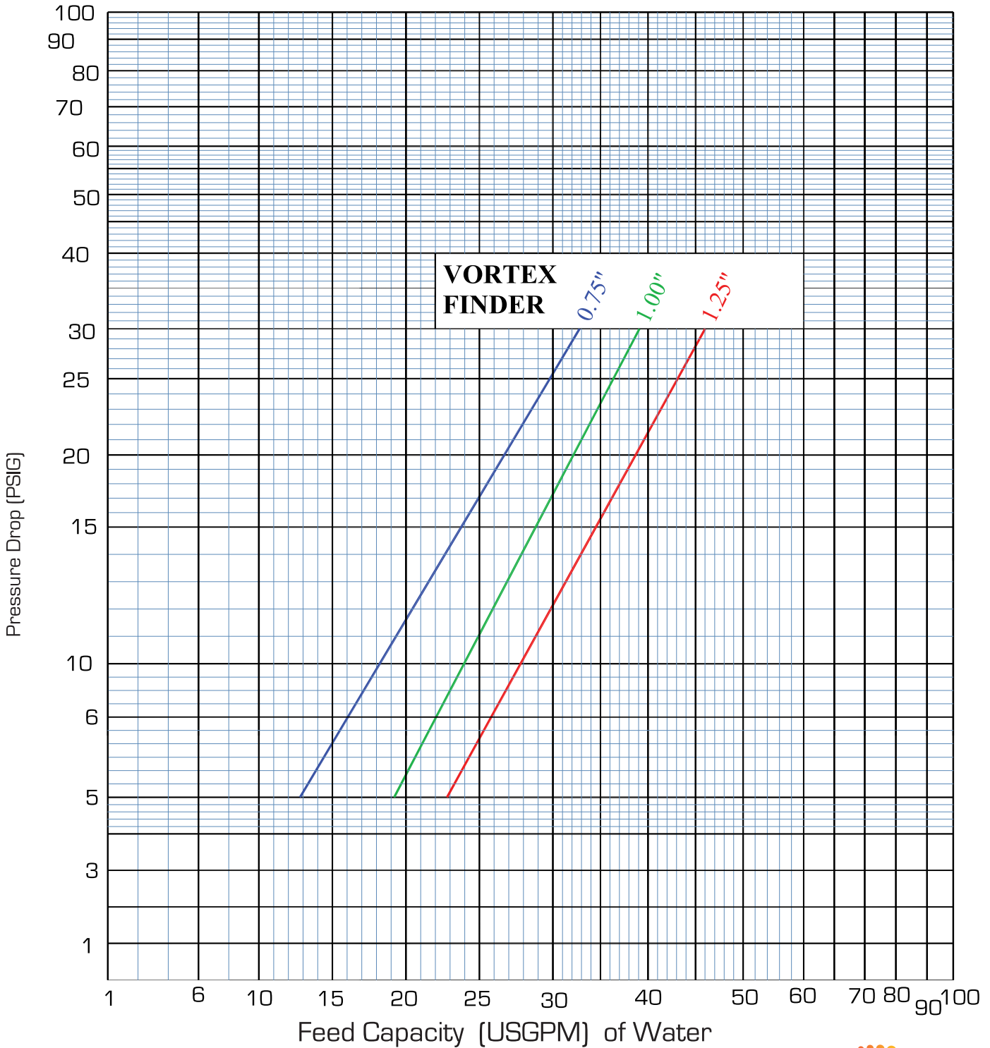
Capacity Curve
